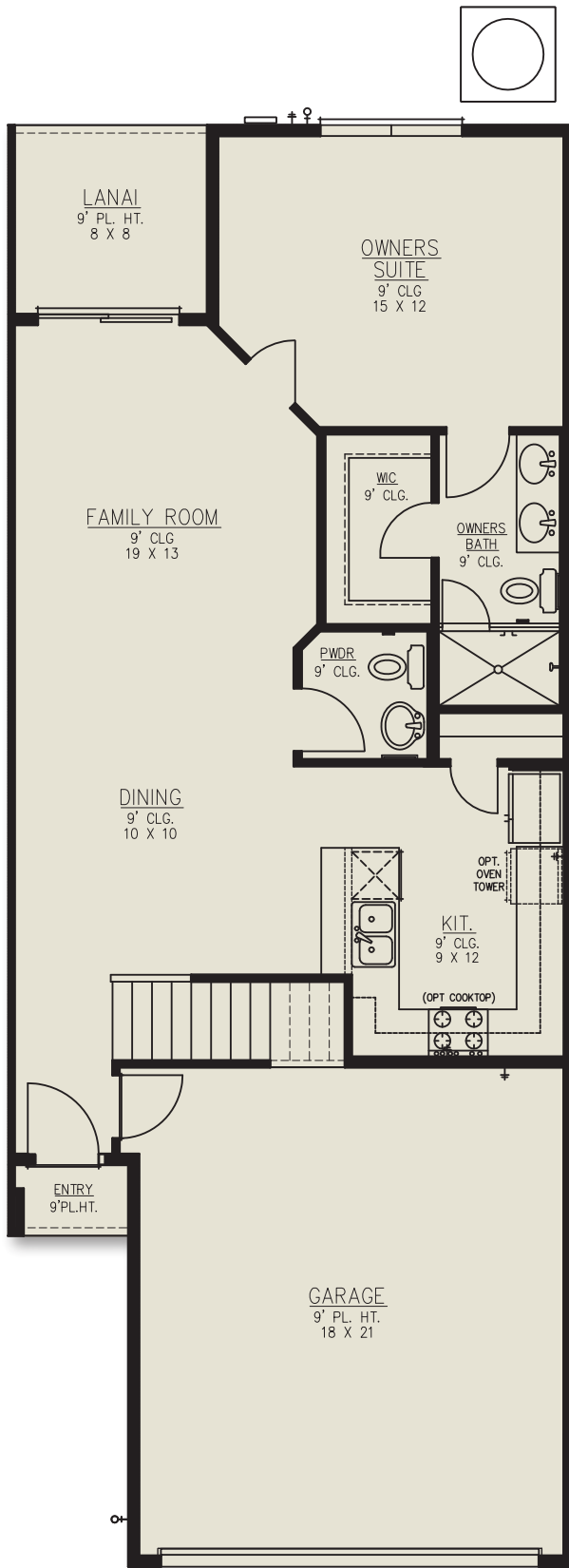
FIRST FLOOR
