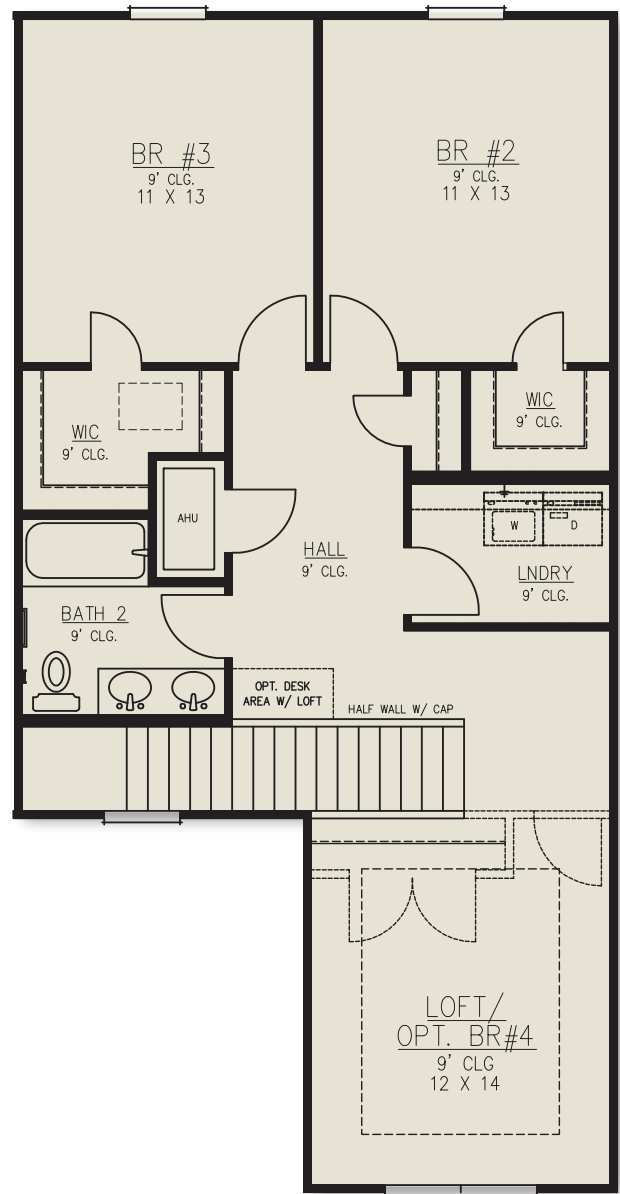
SECOND FLOOR
