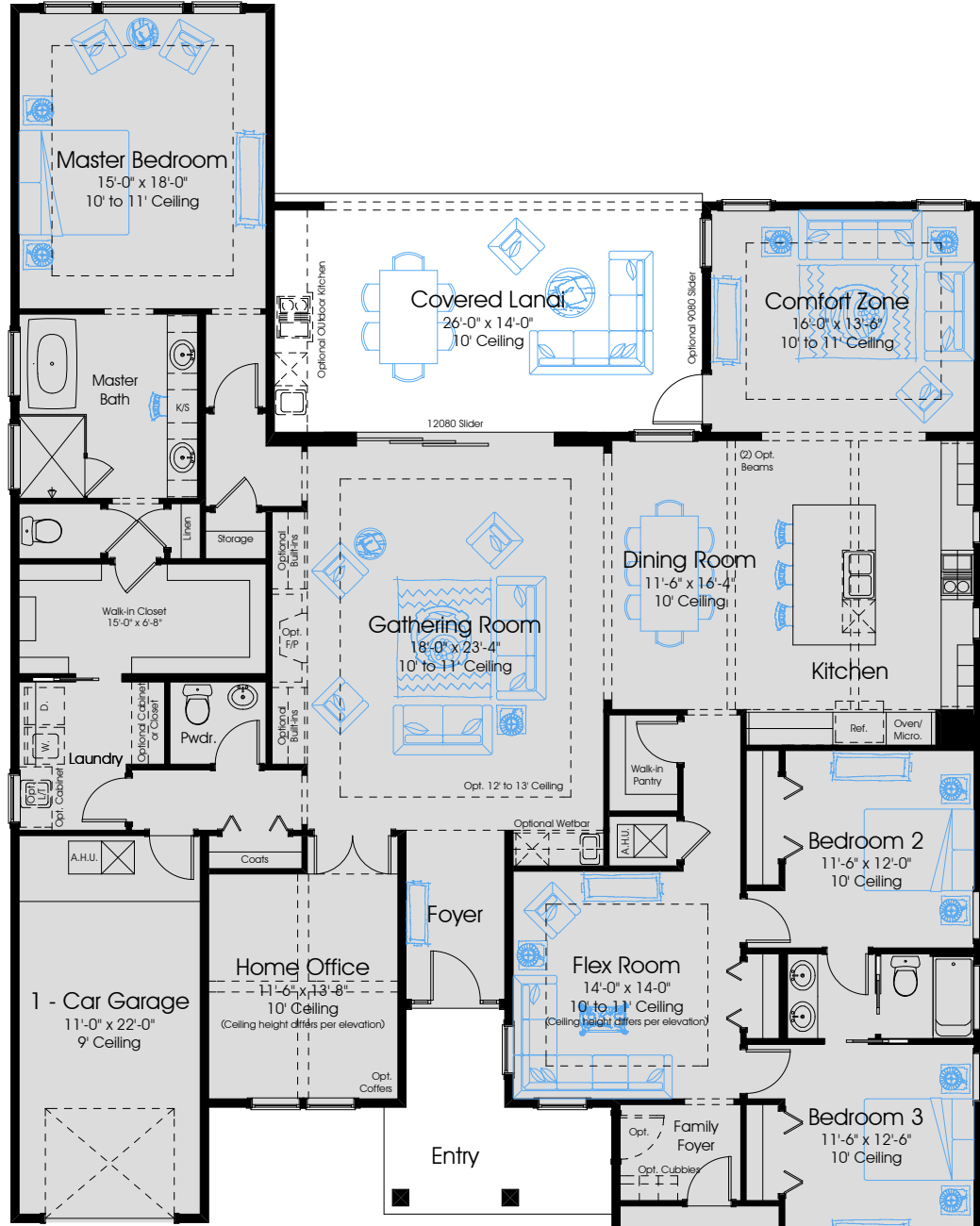
First Floor Plan - Traditional
