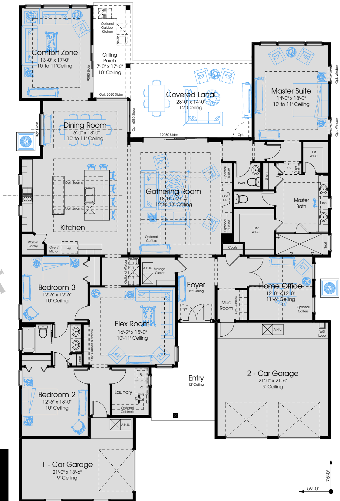
First Floor Plan - Traditional
