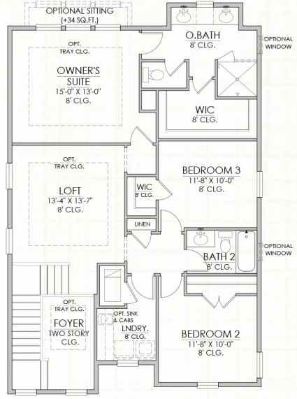
2ND FLOOR PLAN
