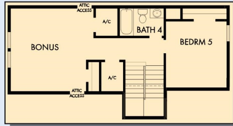
SECOND FLOOR WITH OPTIONAL BONUS WITH BEDROOM 5 AND BATH 4
