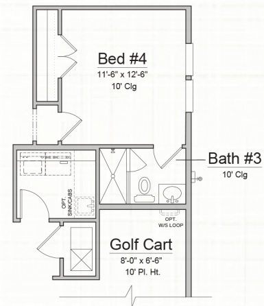
OPTIONAL BEDROOM 4 & BATH 3 (+47 HTD. SQ.FT.)
